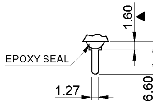
TERMINAL DETAIL
